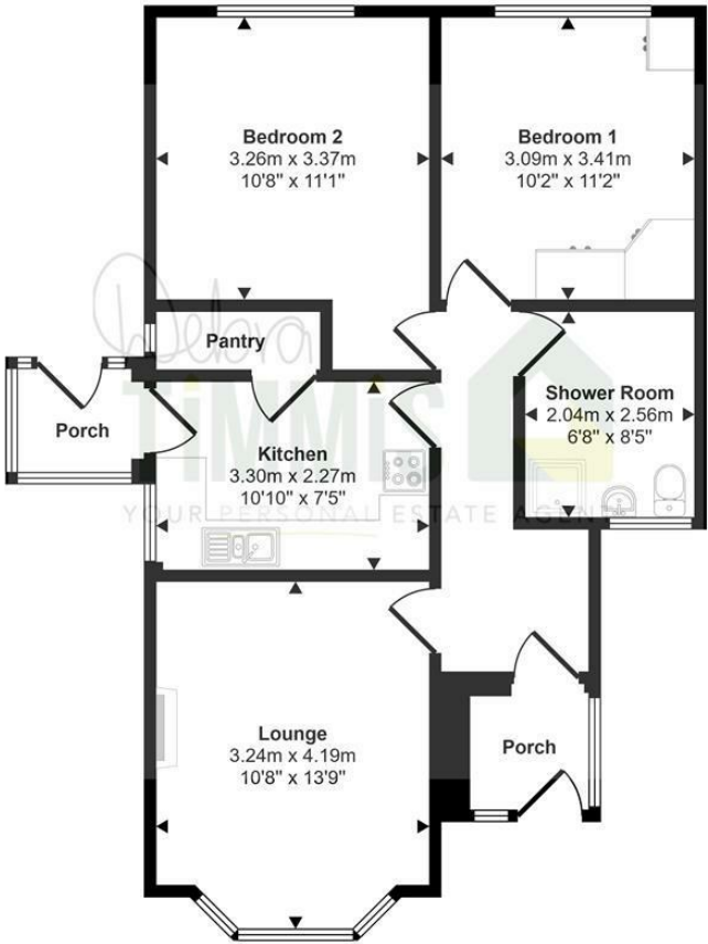
Floorplan
