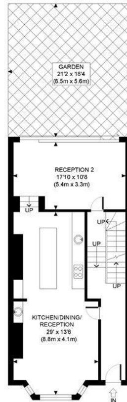
GROUND FLOOR GROSS INTERNAL FLOOR AREA 692 SQ FT
